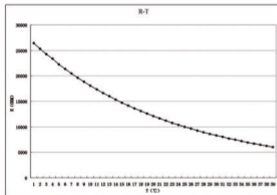
Temperature graph against resistance
